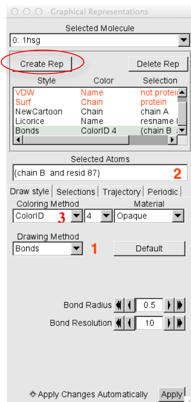
Figure 2. The VMD graphical Representation window. Note that (1) the drawing method defines which graphical representation is used and (2) the selection determines which part of the molecule is drawn, and (3) defines the color it is displayed with. You are encouraged to explore different drawing styles ( Drawing Methods - labeled 1) including Licorice , Tube and NewCartoon
