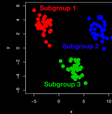
3 Groups
