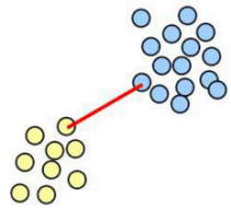
single-link
