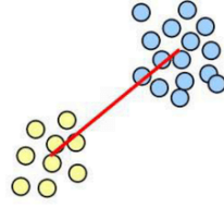
average-link
