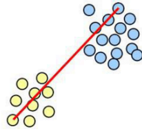
complete-link
