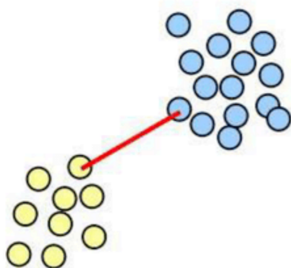
single-link
