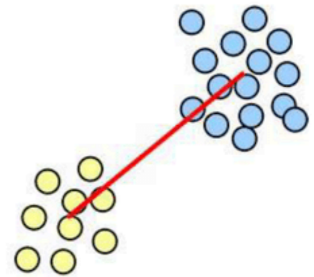
average-link
