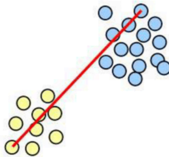
complete-link
