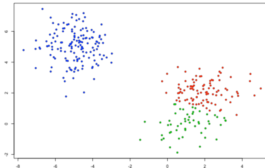
Total Within SS = 533.630315419879
