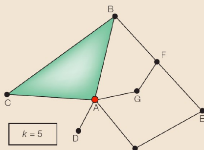
a Undirected network
